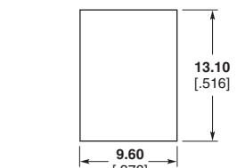
Recommended Panel Cutout Max. Panel Thk. 1.7 [0.067]
